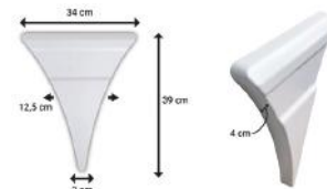
Part No. 20000245 Without cutout for sidemarker light Part No. 20000248 With cutout for sidemarker light MUDGUARD STRINGS Set of 2pc, suitable for Scania Nextgen. € 219,00 excl. VAT / € 264,99 incl. VAT
