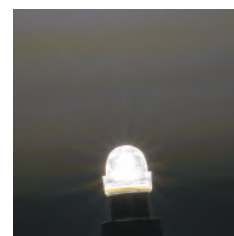
Part No. 46350283 – White BA9S - 1 HI-POWER SMD LED Multivolt 24-32V, set 2pc € 5,50 excl. VAT / € 6,66 incl. VAT
