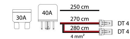
Autoline connection kit, 2 x DT 4
