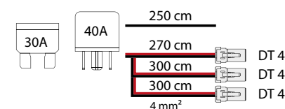
Autoline connection kit, 3 x DT 4
