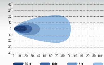
Wide light pattern.
