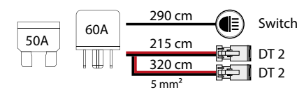
Autoline connection kit, 2 x DT 2
