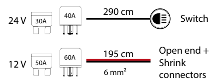
Autoline connection kit, open cable ends
