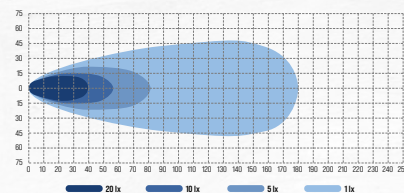
BULLBOY PROLINE SINGLE 1010 23900 lm, 432 W.
