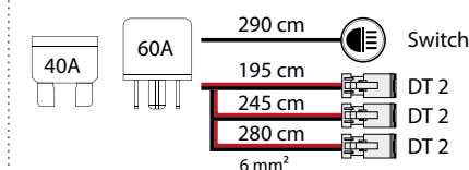
Autoline connection kit, 3 x DT 2
