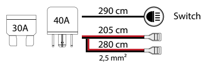
Autoline connection kit, 2 x blade terminals
