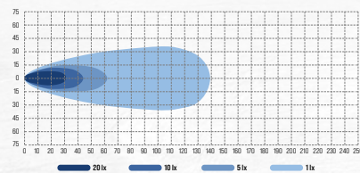
BULLBOY PROLINE SINGLE 578 12600 lm, 240 W.
