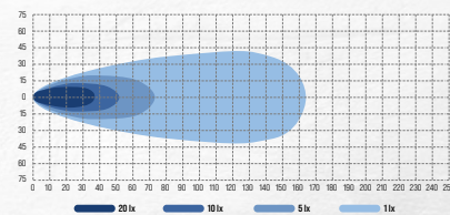
BULLBOY PROLINE SINGLE 793 17500 lm, 336 W.
